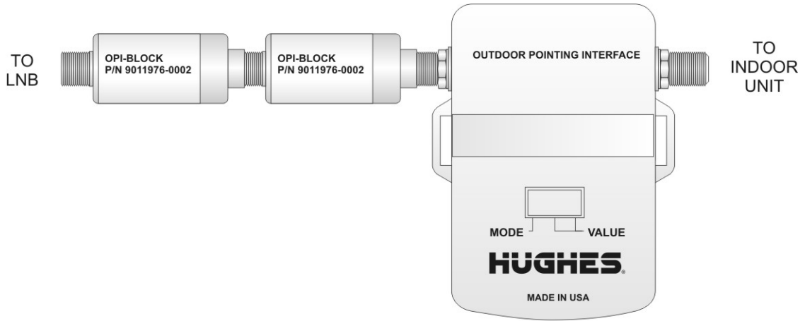
Figure 1. Configuring the OPI and 22 kHz filters in series
